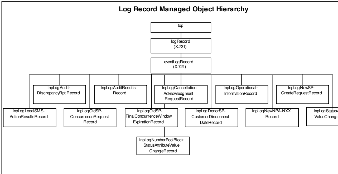
Exhibit 3 . Log Record Managed Object Hierarchy
